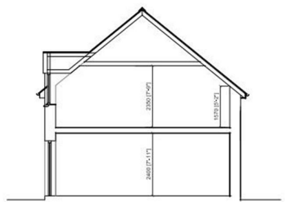
Section scale 1:100
