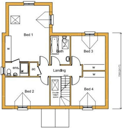
First Floor plan scale 1:100
